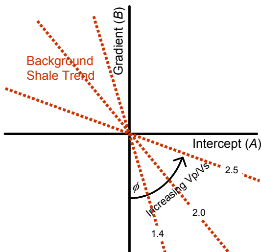
Figure 3: Schematic AVO crossplot showing how increasing V_p/V_s is related to the angle the background shale trend makes with the negative B axis. After Castagna and Swan (1997).
