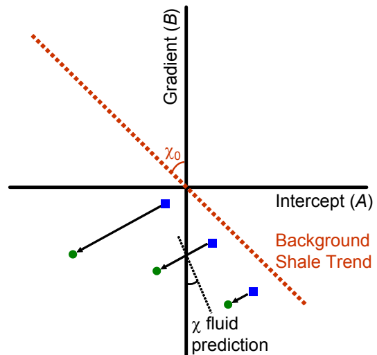
Figure 2: Schematic AVO crossplot showing shale-brine sand (blue squares) and shale-gas sand (green circles) responses.
