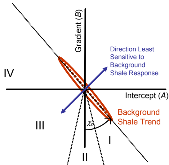
Figure 1: Schematic AVO crossplot showing regions corresponding to Class I-IV reflections. The background shale trend plots at an angle of \chi_0 from the negative B axis.
