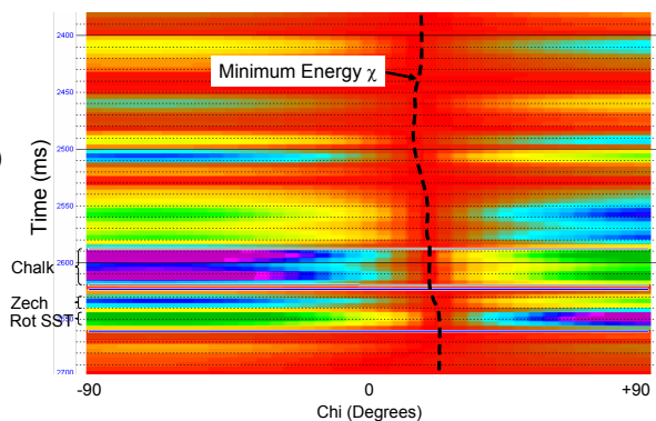
Figure 4: EEI logs as a function of \chi . Changes in the minimum energy \chi angle with depth are indicated by the dashed line.
